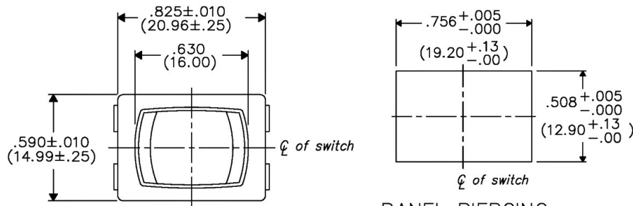
PANEL PIERCING
