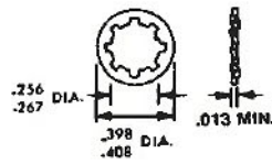
Internal Tooth Lockwasher
