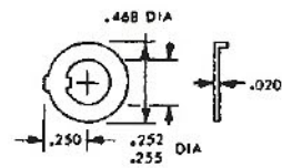
Std. Locking Ring
